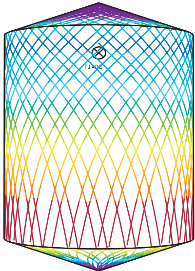
D4.6m H5.5m, Toftejord TJ40G, 4 x ø7.3 mm, Time = 2 min., Water consumption = 700 l
