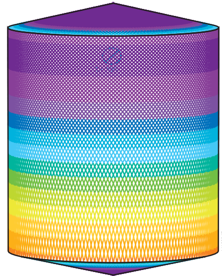
D4.6m H5.5m, Toftejord TJ40G, 4 x ø7.3 mm, Time = 16 min., Water consumption = 5600 l
