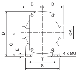
Figure 1. Horizontally Ported
