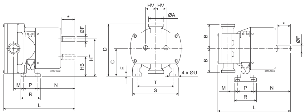
Figure 2. Vertically Ported
