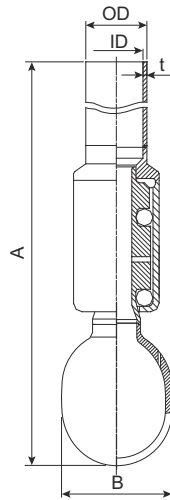
Figure 2. Weld-on
