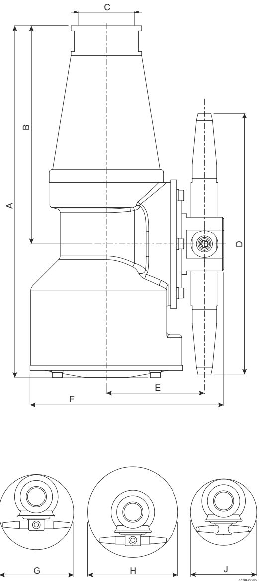
4 nozzle version
